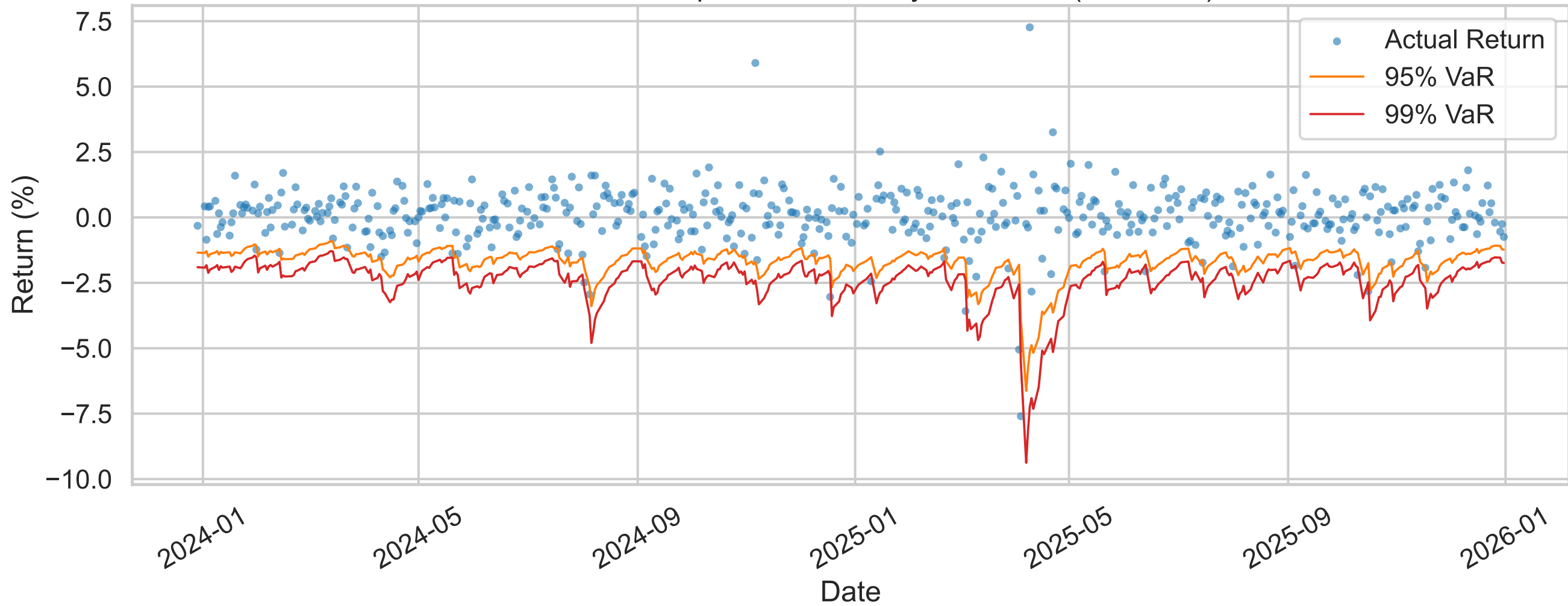
XLF Out-of-Sample Returns vs Dynamic VaR (EGARCH)
